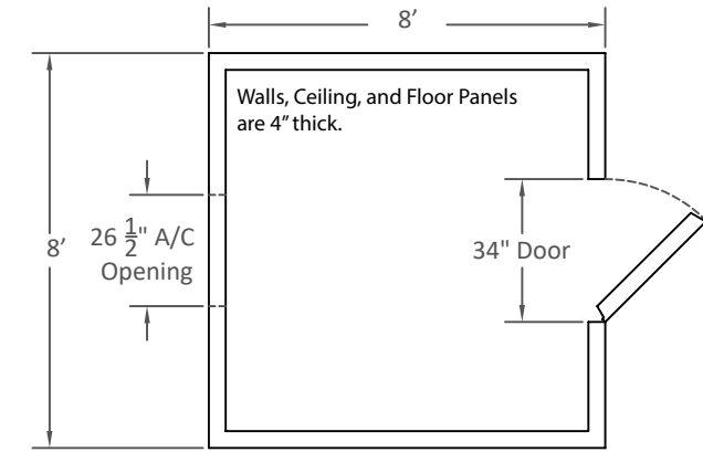
Cooler Nominal Dimensions shown - Contact us for Actual Dimensions
